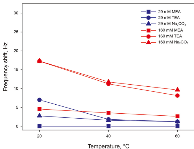
Fig. 6. Frequency shifts as a function of temperature for alkali solutions with 29 and 160 mM of MEA in 50 mM \text{Ca}^{2+} , of TEA in 50 mM \text{Ca}^{2+} , and of \text{Na}_2\text{CO}_3 in Milli-Q water, all at pH 9.5.
