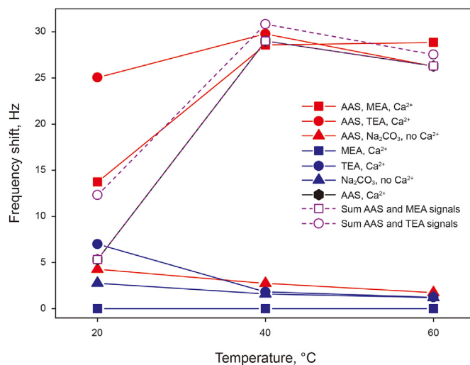
Fig. 7. Comparison of frequency shifts as a function of temperature for solutions of 0.15 wt% AAS in presence of 29 mM MEA in 50 mM \text{Ca}^{2+} , of 29 mM of TEA in 50 mM \text{Ca}^{2+} , and of 29 mM \text{Na}_2\text{CO}_3 in Milli-Q water, the same solutions without AAS, and in 50 mM \text{Ca}^{2+} , all at pH 9.5.
